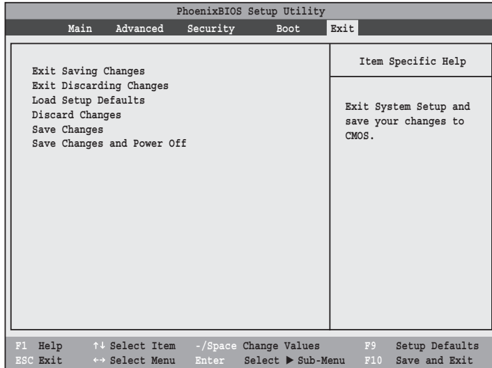
Figure 20. Exit Menu
